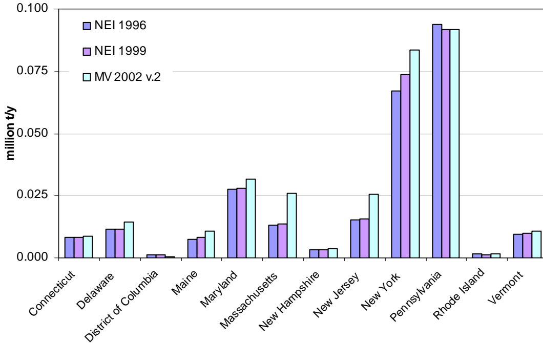
Figure 3-12. 2002 MANE-VU state NH 3 inventories
